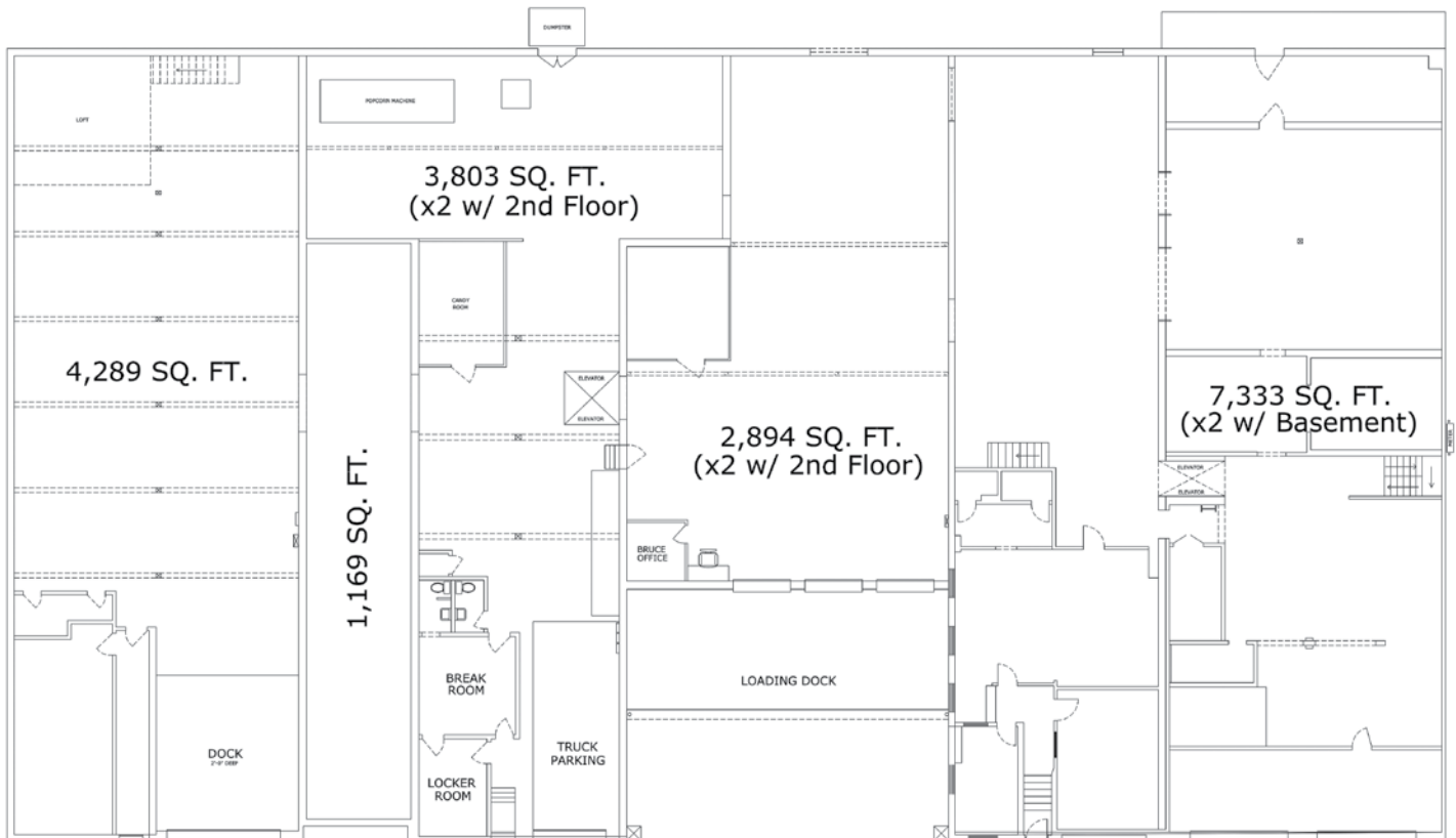
1ST FLOOR LAYOUT
